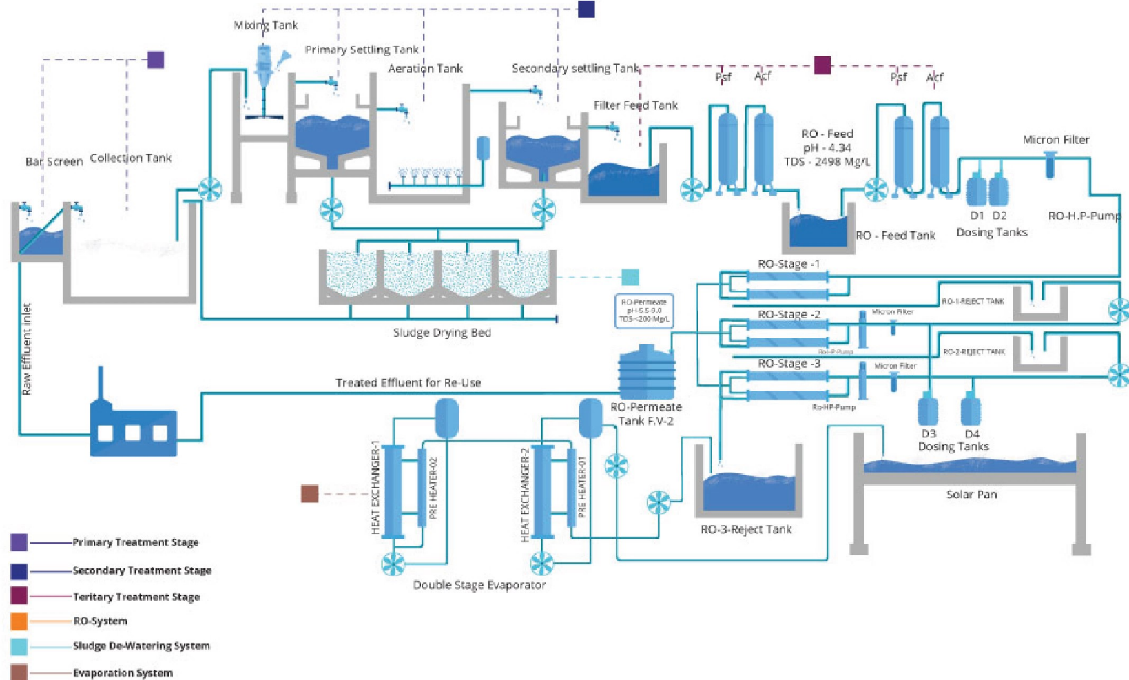
ZERO LIQUID DISCHARGE PLANT
