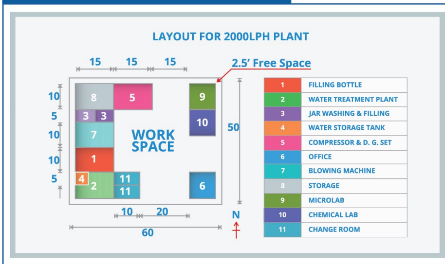
PLANT LAYOUT (FOR EXAMPLE 2000 LPH PLANT)
