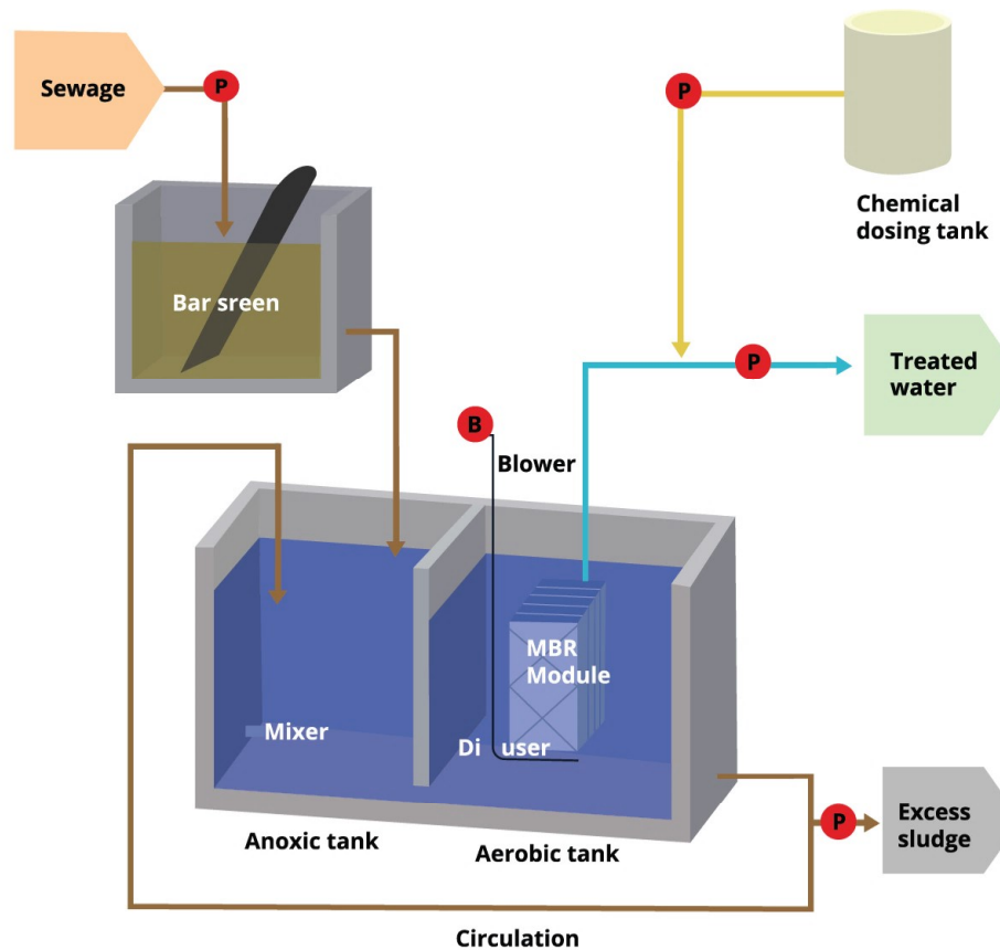
General Process Flow Diagram
