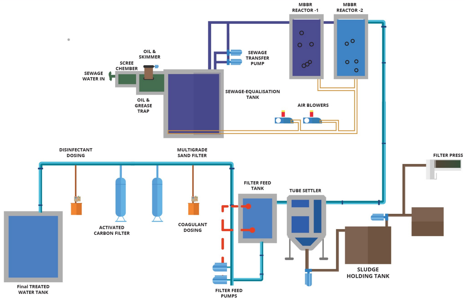
Typical flow sheet diagram of STP
