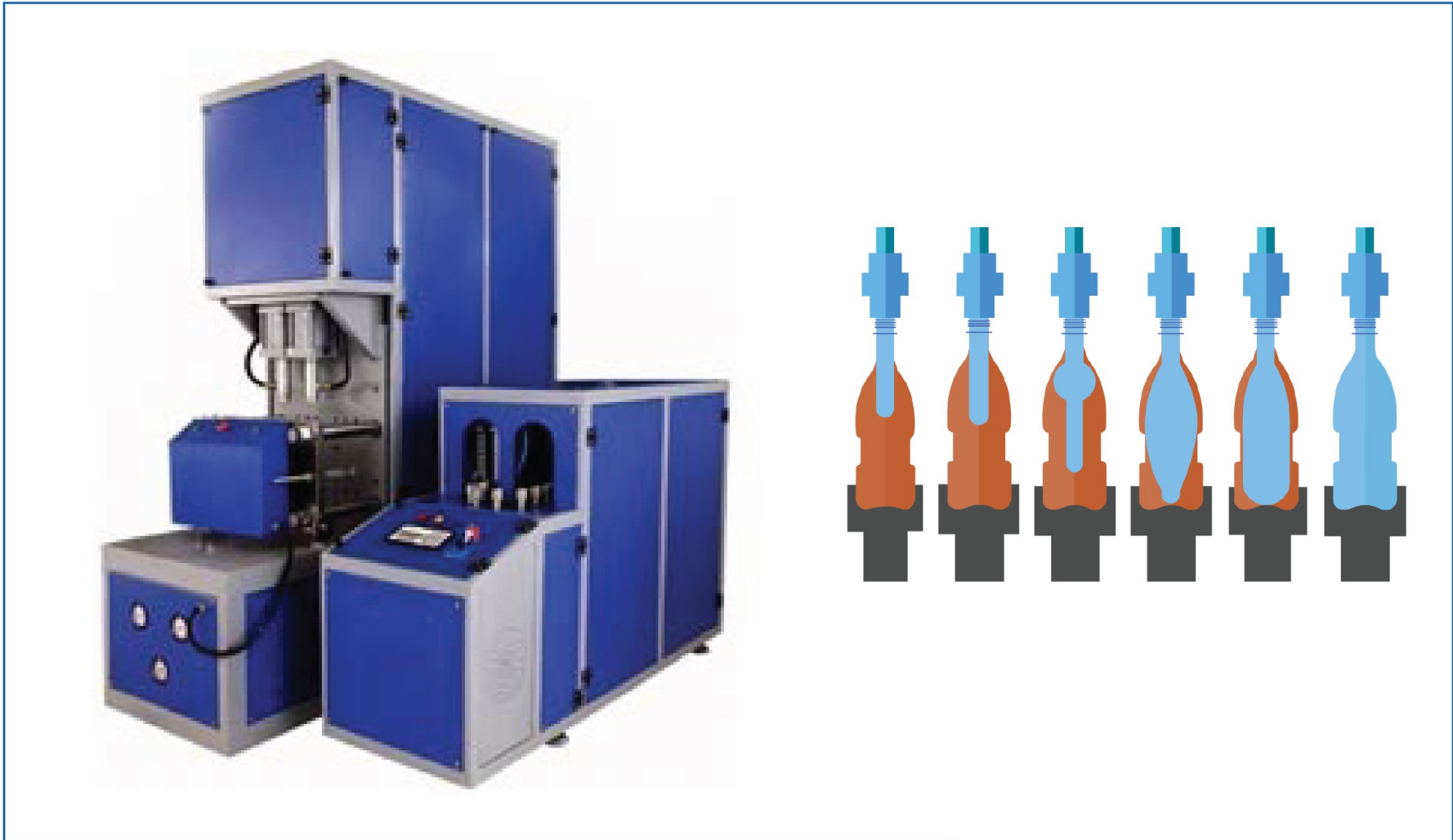
PET BLOW MOULDING MACHINE
