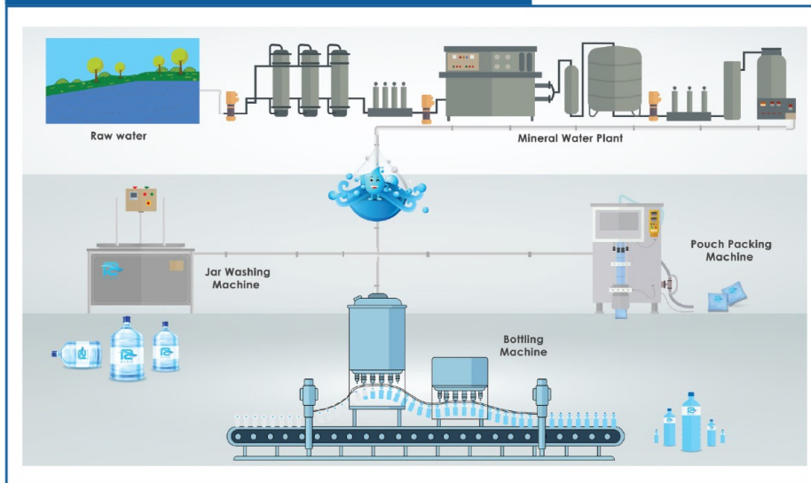
MINERAL WATER TURNKEY PROJECT DIAGRAM
